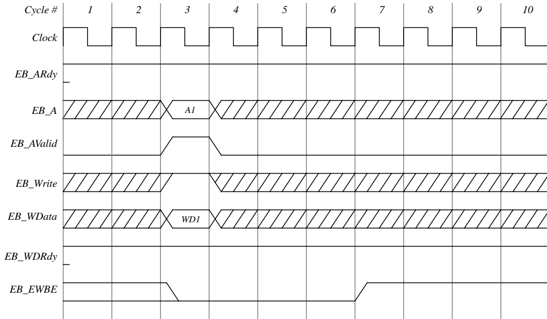
Figure 2-13 Example of EB_EWBE signalling when no wait states on address/data.
